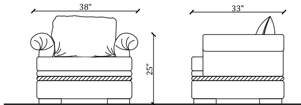
SINGLE SEATER SOFA FRONT VIEW
